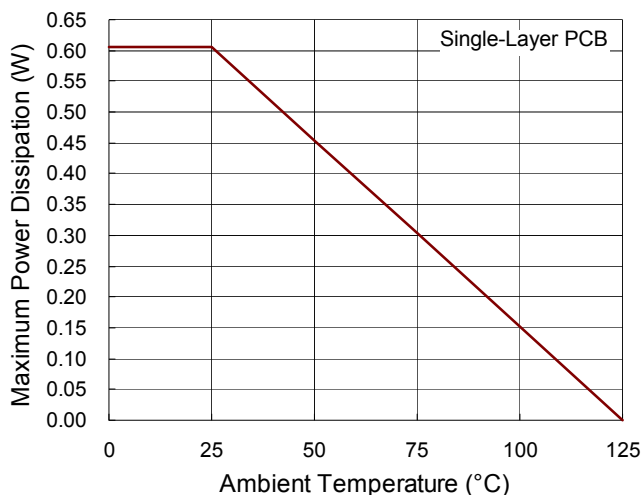
Figure 5. Derating Curves for RT8238B Packages
