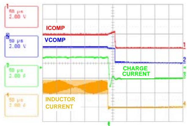
FIGURE 8. CHARGE DISABLE
