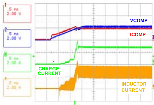
FIGURE 7. CHARGE ENABLE
